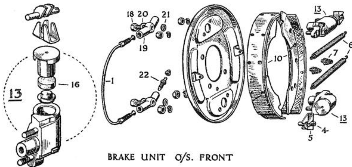
Front Brakes (Above)
