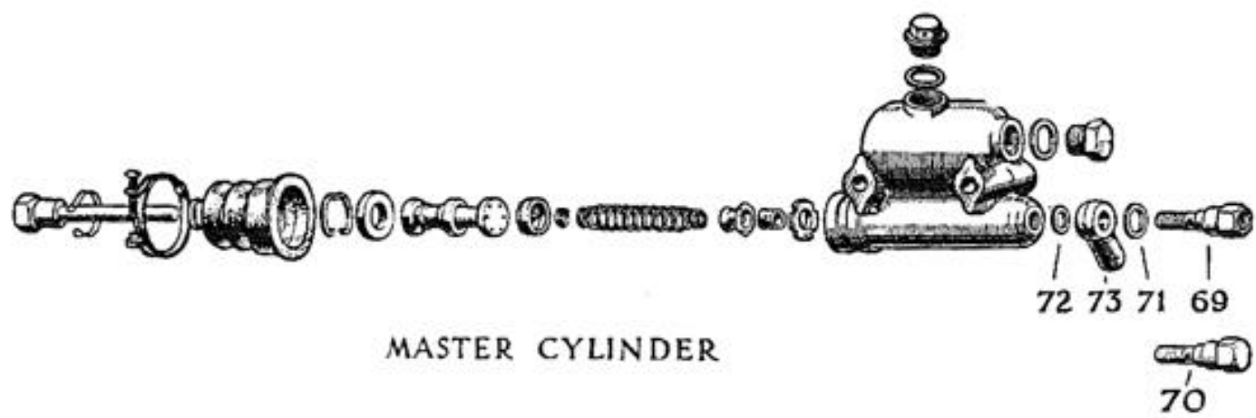
Master Cylinder (Above)
