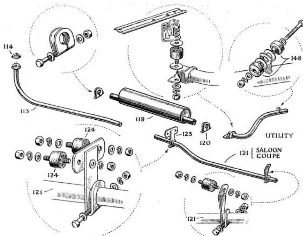
Exhaust System (Above)
