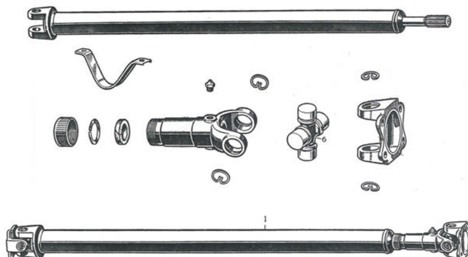
Propellor Shaft (above)
